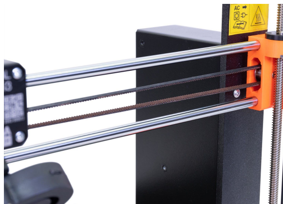
Pict. 48 - A properly-tightened X-axis belt
