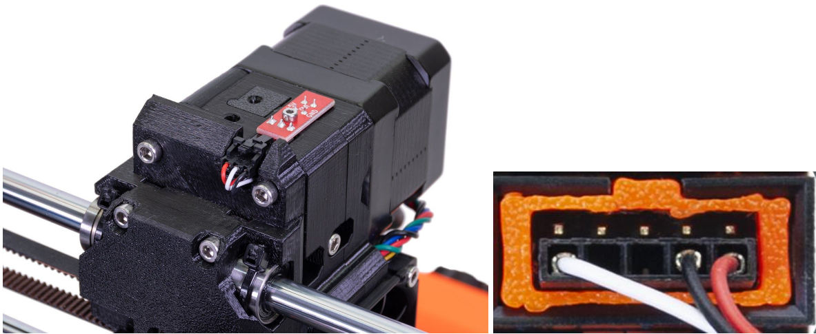
Pict. 38 - Properly connected and seated filament sensor
