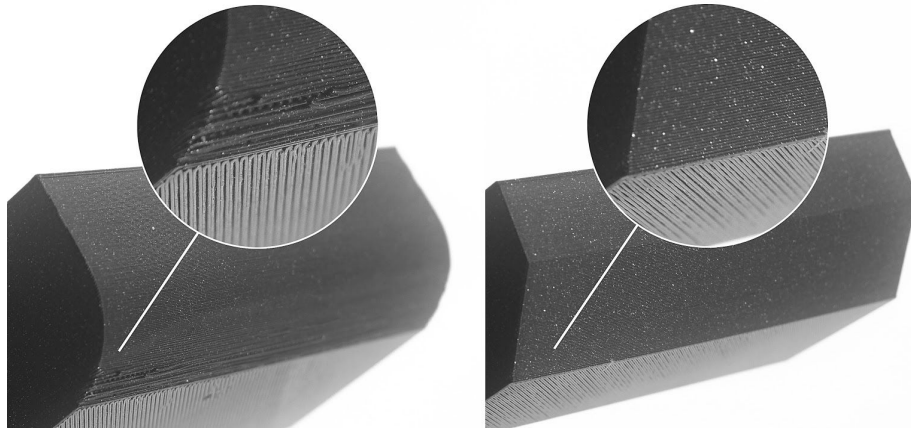
Pict. 28 - Fillet (left) vs chamfer (right)
