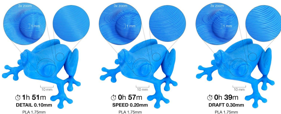
Pict. 19 - Print quality vs print time
