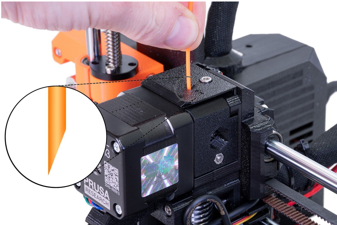
Pict. 9 - Loading the filament into the extruder
